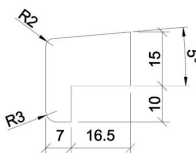
Figure 2 – MDF Bead – Option 1
